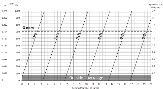
PV Compact DN20, 5-30 kPa
