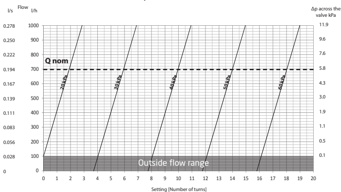
PV Compact DN15, 20-60 kPa
