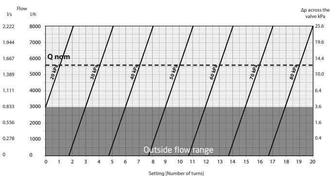
PV Compact DN40, 20-80 kPa
