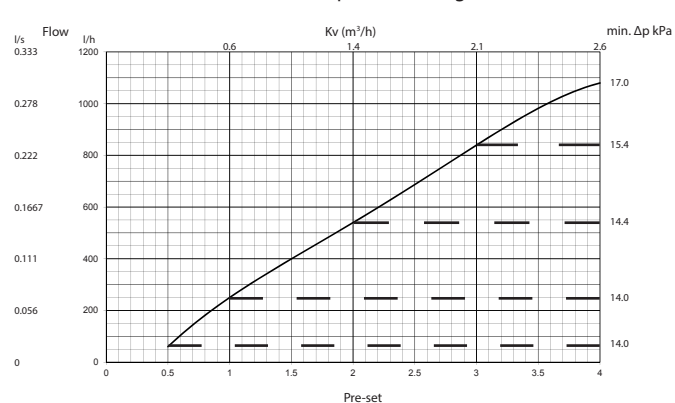
SIGMA Compact DN15 High
