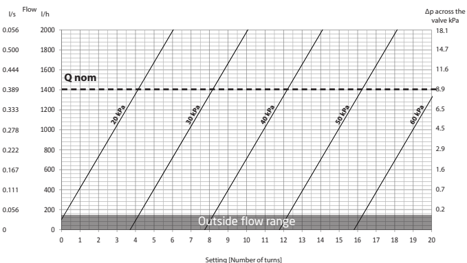
PV Compact DN20, 20-60 kPa
