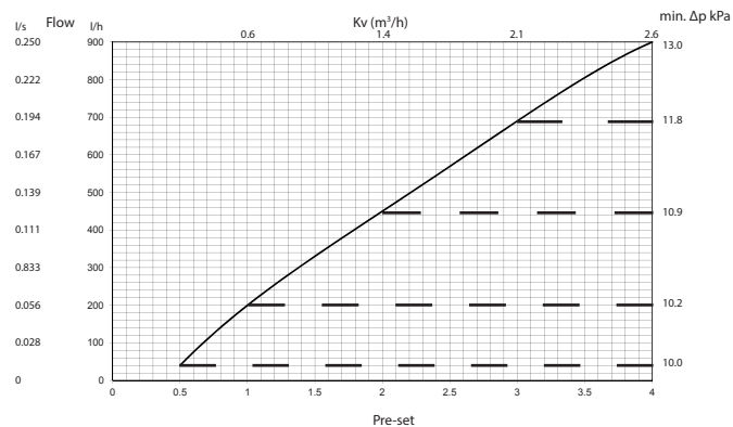
SIGMA Compact DN15 Low
