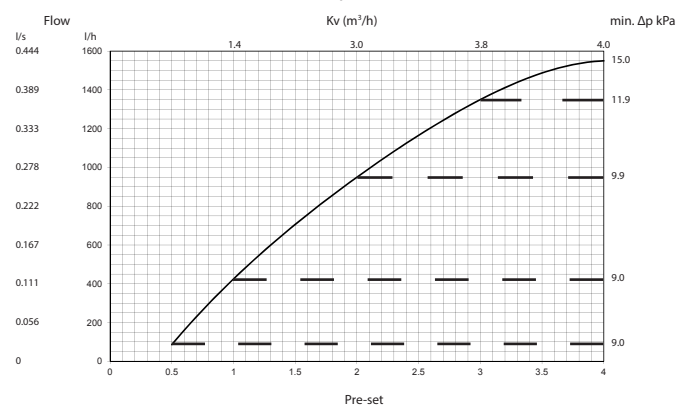
SIGMA Compact DN20 Low
