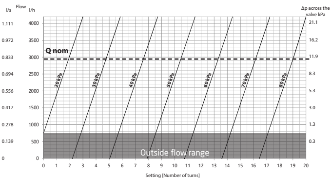
PV Compact DN25L, 20-80 kPa
