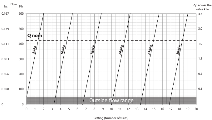
PV Compact DN15, 5-30 kPa
