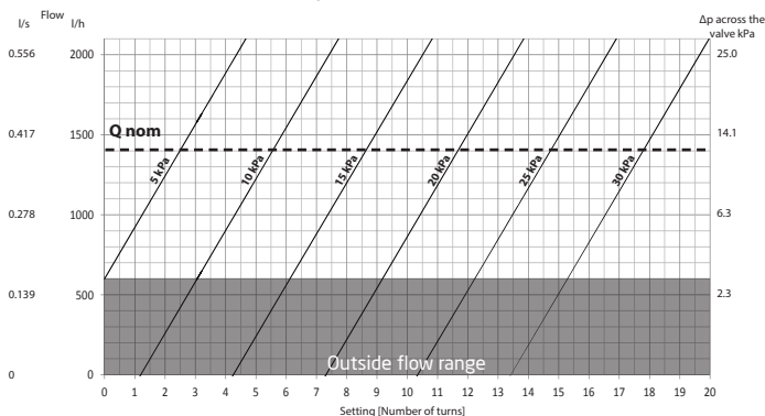
PV Compact DN25, 5-30 kPa
