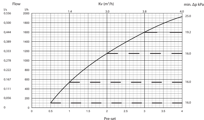
SIGMA Compact DN20 High
