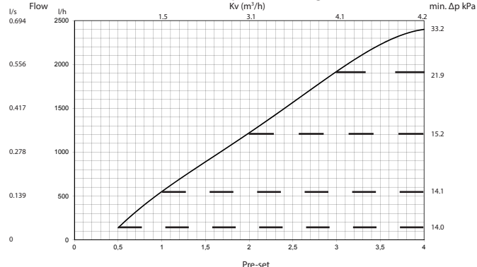
SIGMA Compact DN25 High
