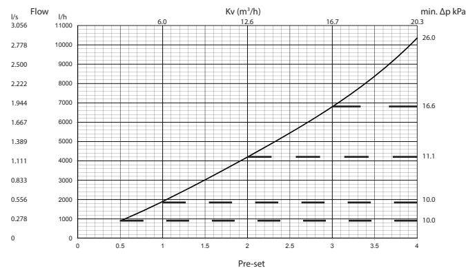
SIGMA Compact DN50
