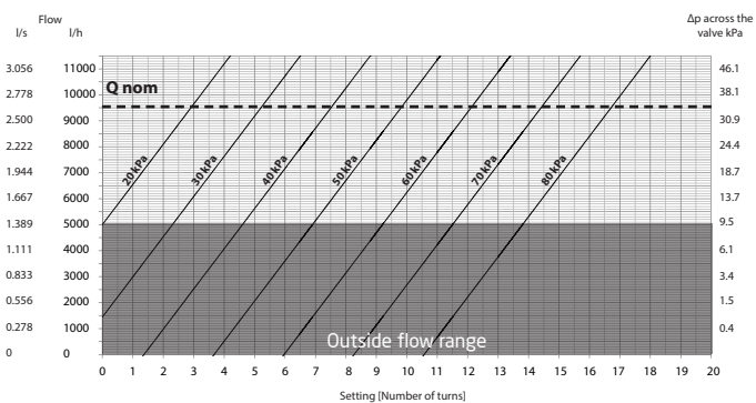
PV Compact DN50, 20-80 kPa
