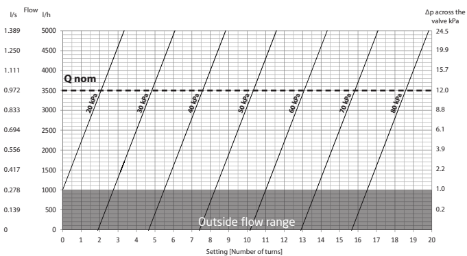
PV Compact DN32, 20-80 kPa
